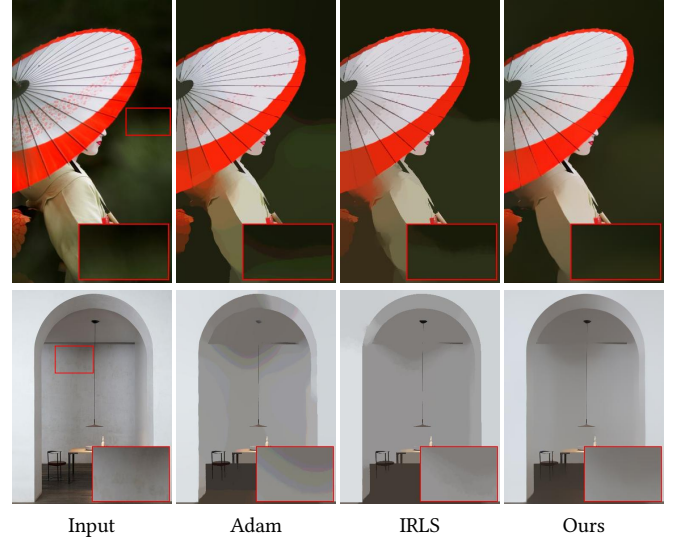
Fig. 5. Comparison between our learned deep neural network and traditional numerical solvers. Compared with the gradient descent optimizer Adam [Kingma and Ba 2015] and Iterative Reweighted Least Square (IRLS) [Holland and Welsch 1977], our results are visually more pleasing which do not have the spurious staircasing structures. Photo courtesy of Tumblr user gaaplite and LucidiPevere Studio.
