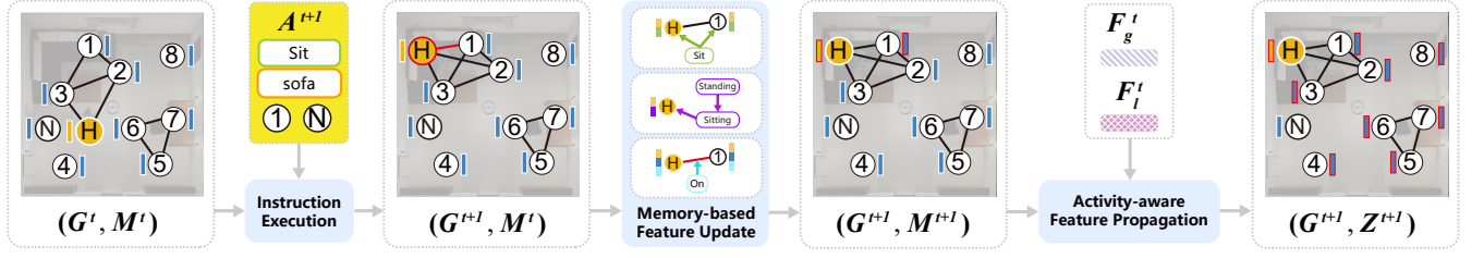
Fig. 6. Instruction execution and scene update: given the current scene graph, memory, and instruction, the instruction is executed to modify the graph, and the node features are updated in the memory-based feature update and then in the activity-aware feature propagation .
