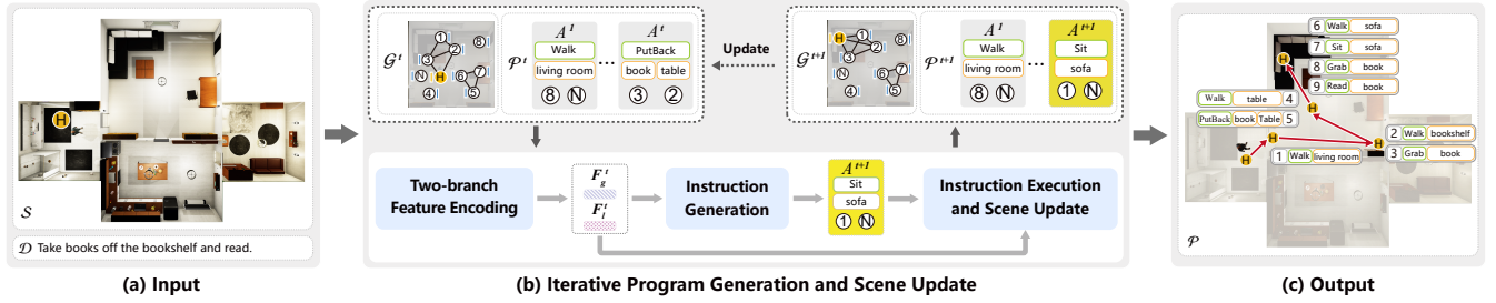
Fig. 2. Overview of our activity program generation method, which takes as input (a) an activity description and a scene with a human agent indicated by the yellow H node. (b) At each iteration, the two-branch feature encoding module first encodes the current state information, including the scene state, partial program, and description of the desired activity, to guide the instruction generation module in predicting the next instruction and target object. Finally, the instruction execution and scene update module updates the scene topology and properties based on the execution of the predicted instruction. The method iterates until (c) the final result with the full program and corresponding motion sequence is generated.
