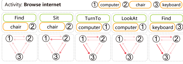
Fig. 7. Attention weights among neighboring objects in the activity-aware feature propagation . Darker colors indicate higher weights.
