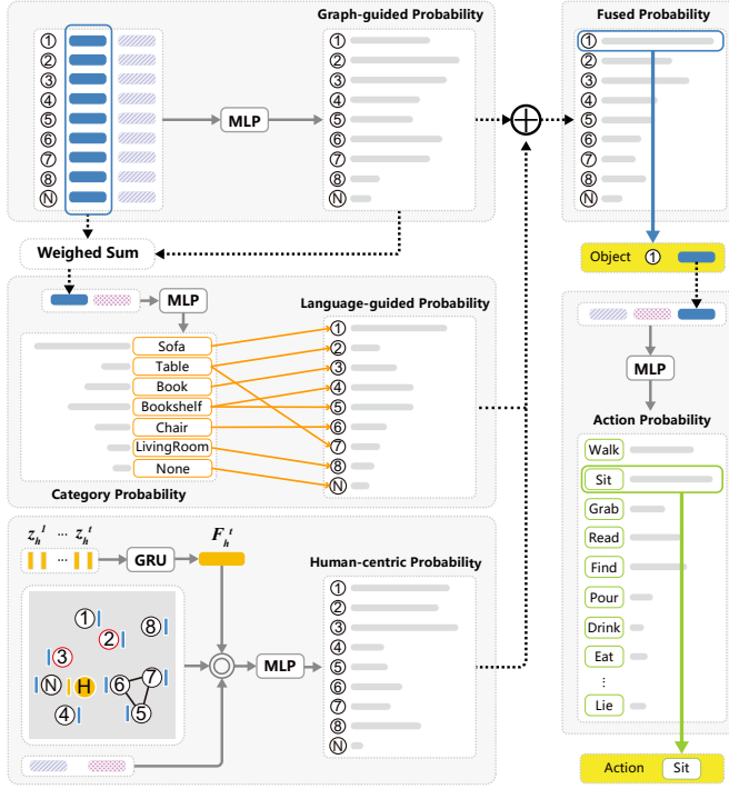
Fig. 4. Instruction generation: a graph-guided probability (top-left), language-guided probability (middle-left), and human-centric probability (bottom-left) are fused together to guide the selection of an object (top-right) and action (bottom-right) that compose a program instruction.
