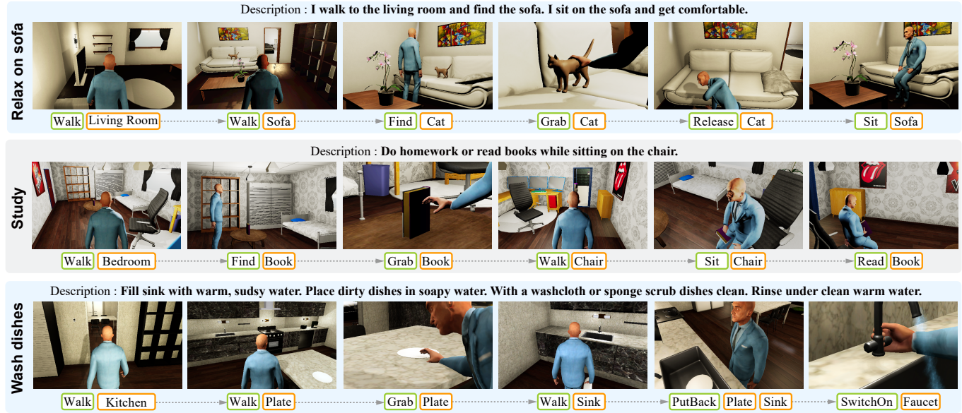
Fig. 1. Our method generates scene-aware activity programs that are highly rational and executable. Here, we show three programs generated by our method, where a virtual avatar is instructed to perform various human activities in different scenes according to the input descriptions.
