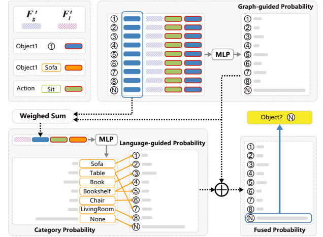
Fig. 5. Prediction of the second object for interaction based on global features and conditioned on the action and object already selected.
