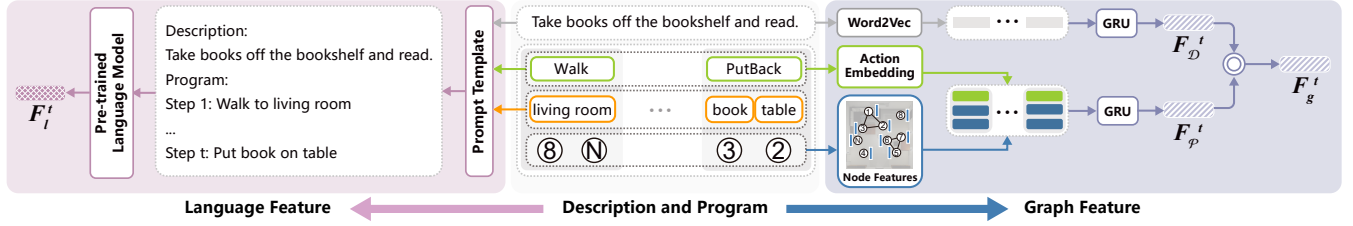
Fig. 3. Two-branch feature encoding: An activity description and partial program (center column) are encoded into a language feature F_l^t (left) through a pre-trained language model, and into a graph feature F_g^t (right) through action embedding and node features extraction.
