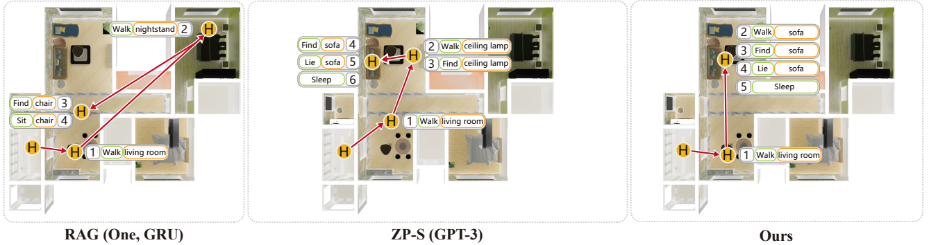
Fig. 13. Qualitative examples showing the generality of our method to scene inputs from different datasets. The sequences of arrows laid over the top views of the scenes show the steps of the activity programs and the locations in the scenes where the activities should take place.
